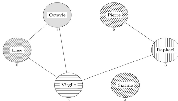
Figure 3. Graphe g_1 coloré
